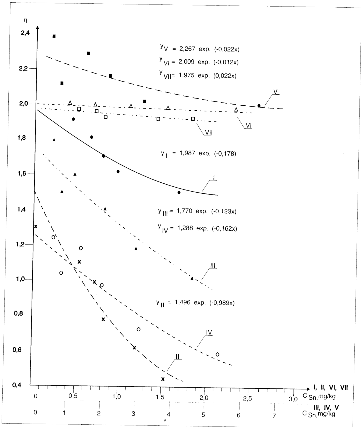
Fig. 6: Influence of Tin Concentration ( C_{Sn}=x ) on Changes of Lustre of Coats ( \eta=y ).
