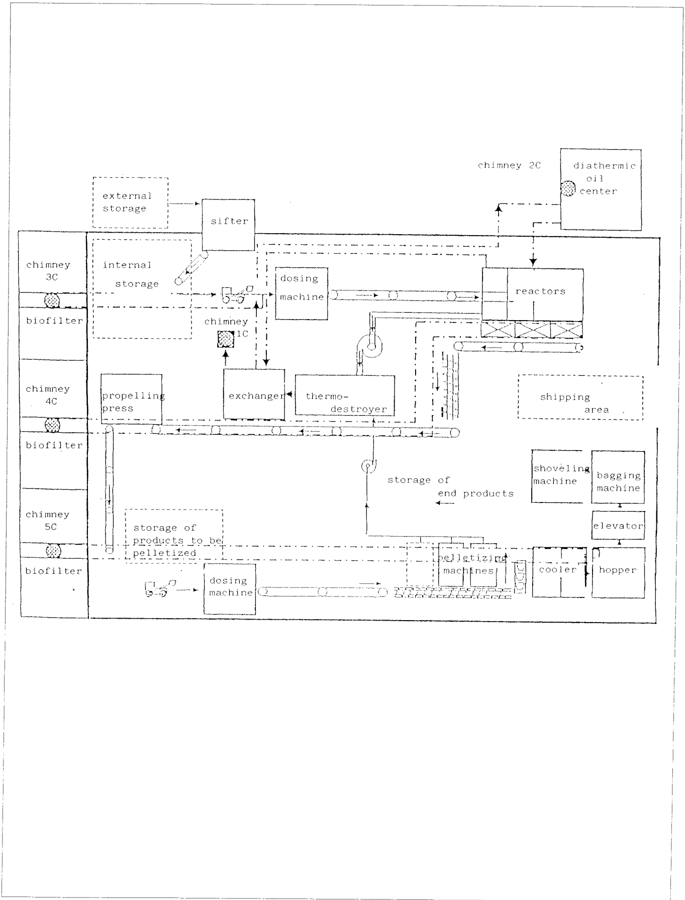
Fig. 1: Production Cycle
