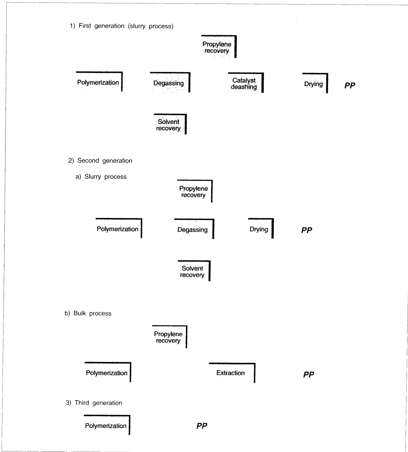
Fig. 3: Schematic Flow Diagram of Various Polypropylene Processes
